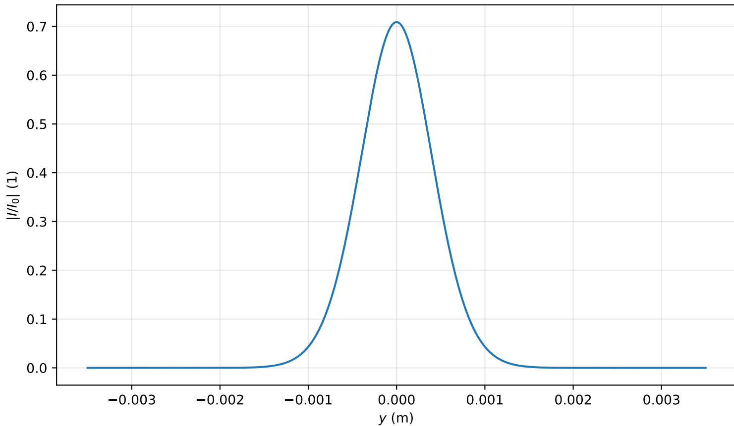
Intensity profile I(x=0, y, z=1.592)/I_0 , P_{in}=0.2P_{cr} , artificial time
